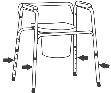
Figure 1: Adjustment areas on commode
